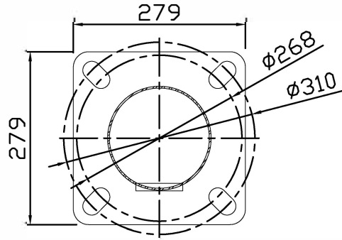
A-A VIEW (3:1)
