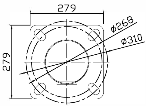
A-A VIEW (3:1)
